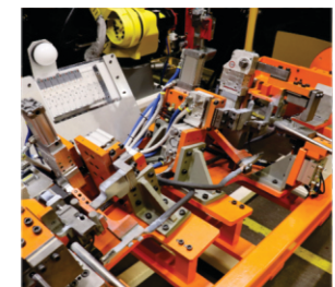
Robotic Fixture
