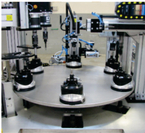
Rotary
