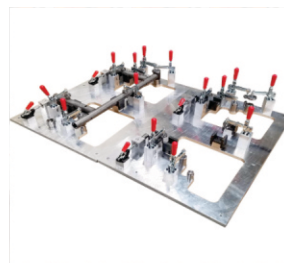
Tooling Fixture
