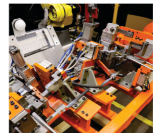
Robotic Fixture
