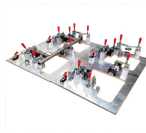
Tooling Fixture
